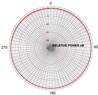
AS-390 (UHF) – AZIMUTH
