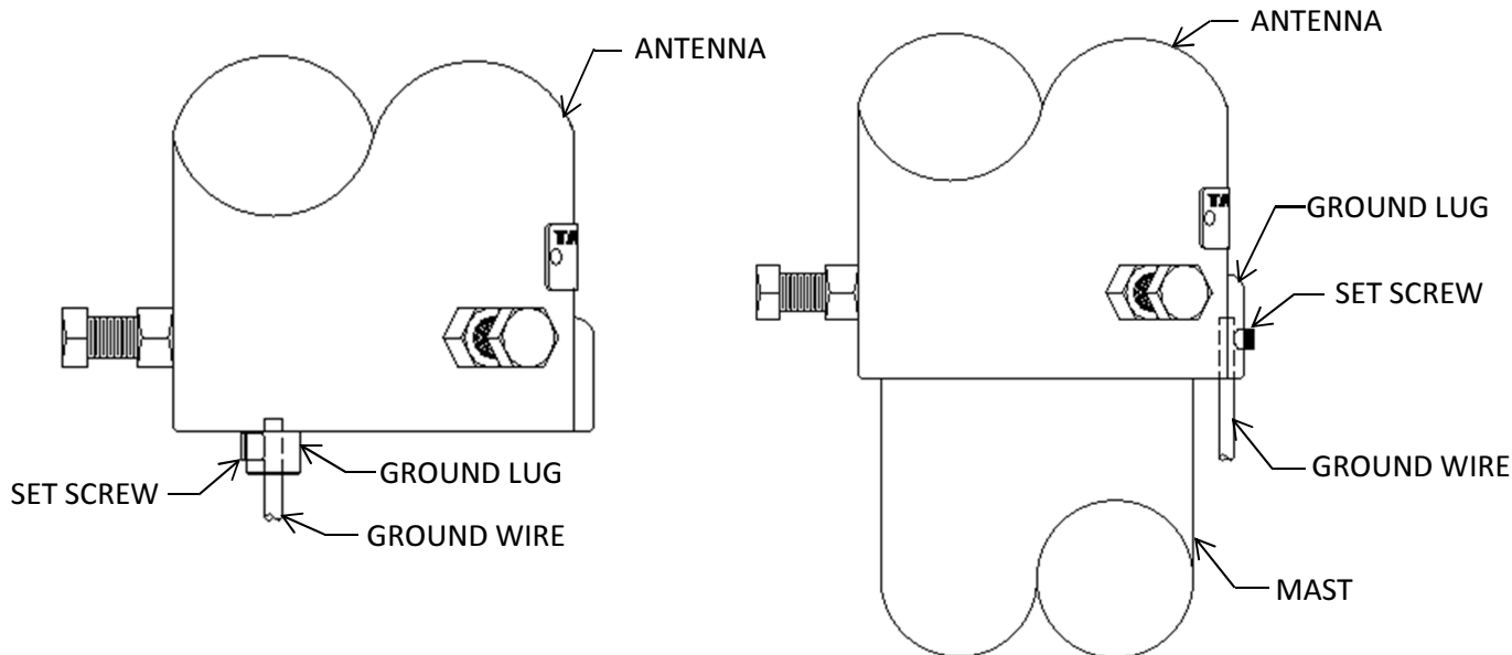
Figure 2: ANTENNA WITHOUT LIGHTNING ROD
